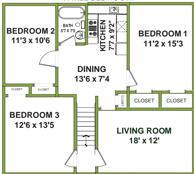
THREE BEDROOM
